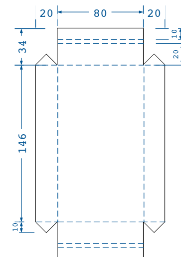
Sliding Shelf
