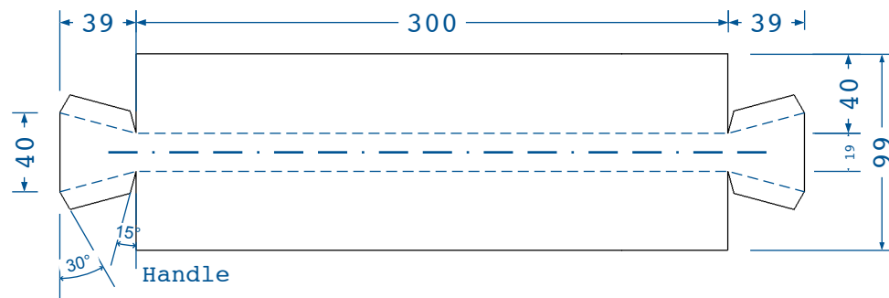
Caddy Body
