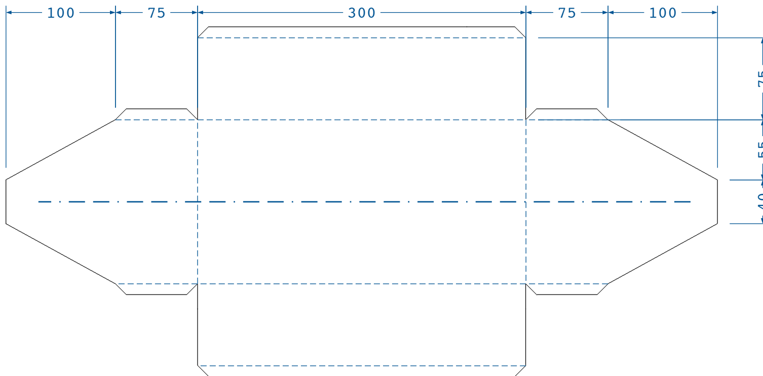
Caddy Body
